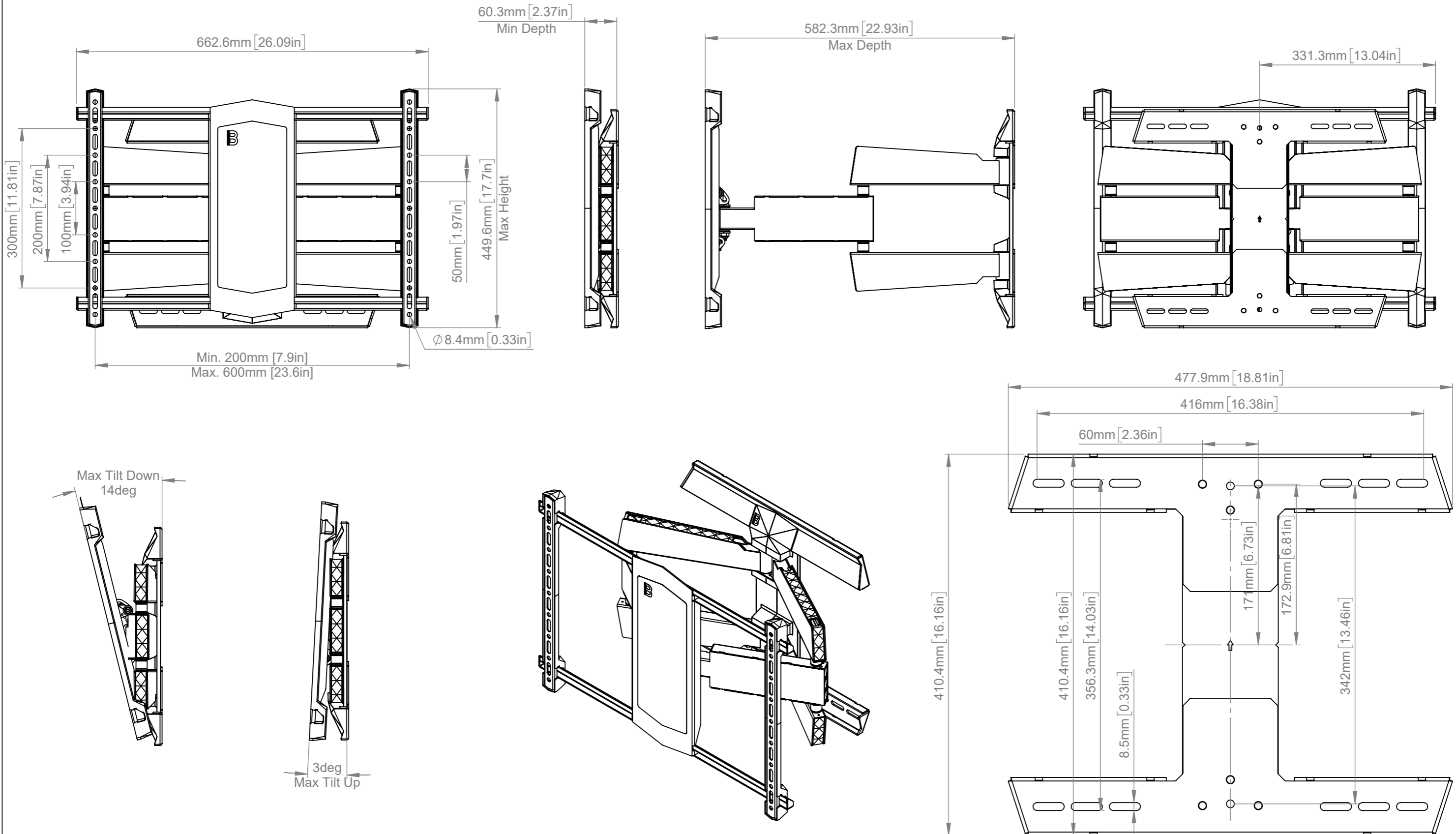
WALL PLATE SCALE 1 : 4
